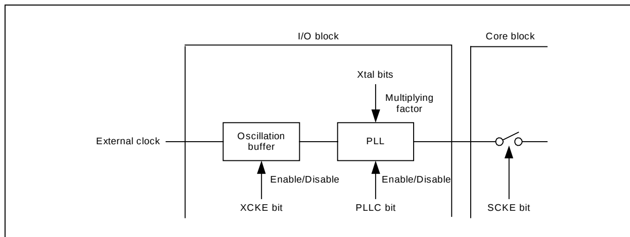
Figure 2.3 Clock Control
